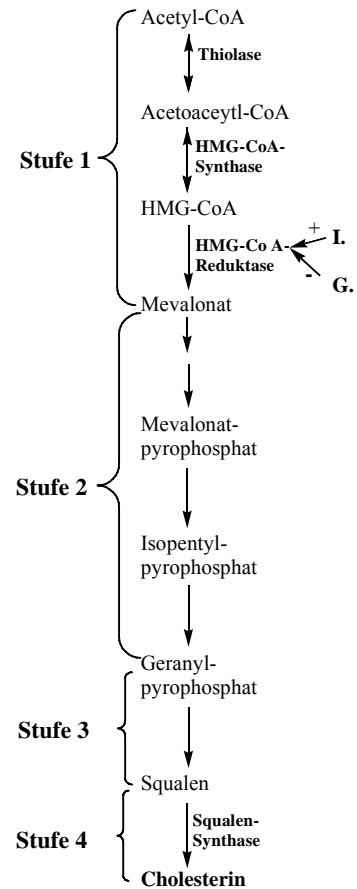
Abb. 4: Cholesterin-Synthese; I.: Insulin, G.: Glucagon [174]
