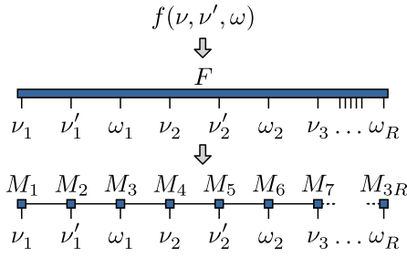
FIG. 4. QTT representation for full vertex function.
