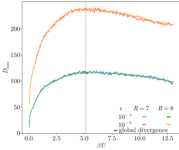
FIG. 7. Maximum bond dimension D_{\max} of the QTT of F_d for different grid sizes and various tolerances set in the TCI construction as a function of \beta U .
