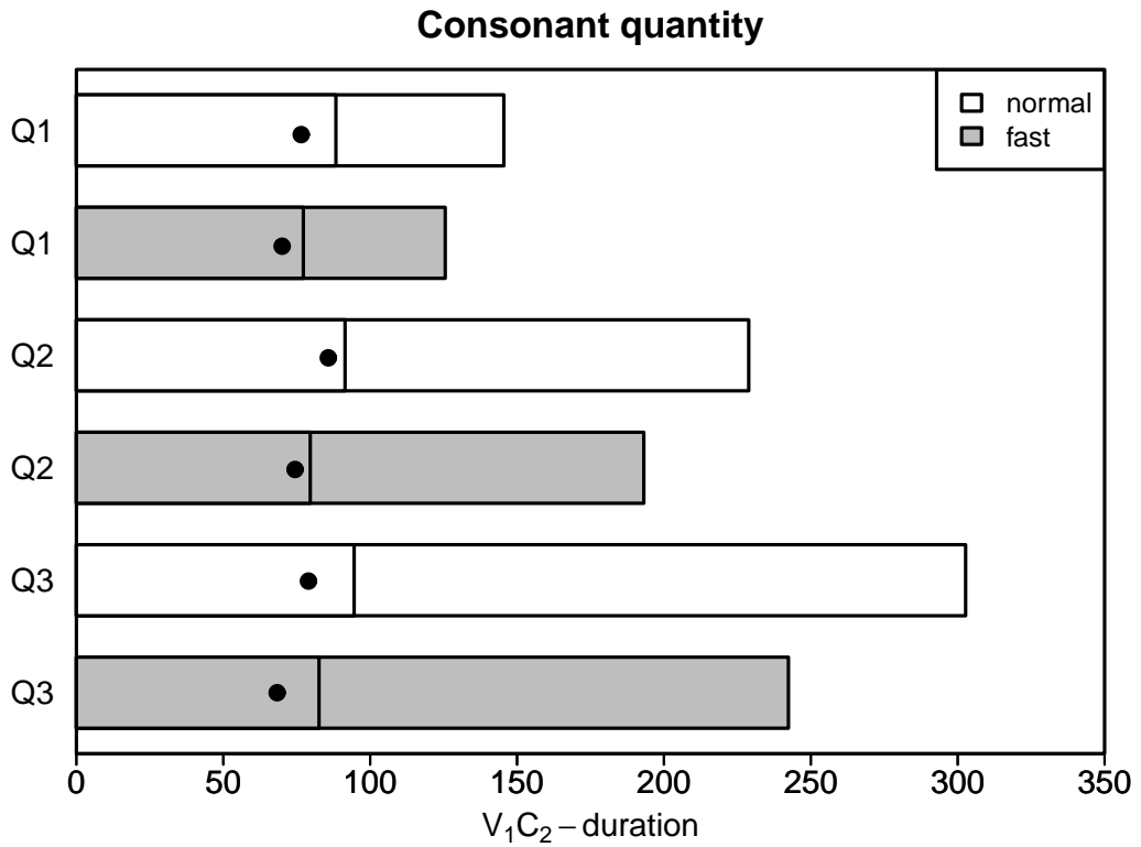
Figure 4.4: The bars show the V 1 C 2 -duration separately for the short (Q1), long (Q2) and overlong (Q3) quantity degree for normal (white bars) and fast (grey bars) speaking rate for CQ-words. The lines indicate the border between V 1 and C 2 . The dots mark the mean value of T abs .
