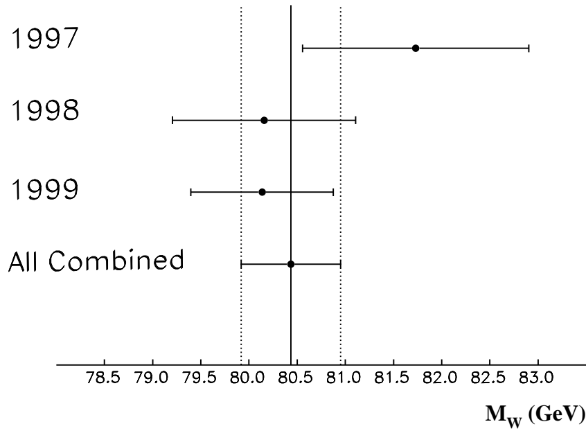
Figure 8.12: Results of M_W measurements in the fully leptonic channel using all data recorded in the years 1997–1999 at center-of-mass energies in the range from 183 GeV to 202 GeV.
