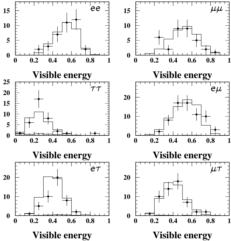
Figure 5.6: Distributions of visible energy scaled to the center-of-mass energy, R_{\text{vis}} , for the six di-lepton classes selected as W^+W^- \rightarrow \ell\nu\ell'\nu_{\ell'} events. The data are shown as the points and the error bars denote the statistical errors. The total Monte Carlo expectation is shown as the histogram with the non- l^+ l^- \nu \nu' background contribution shown by the hatched histogram.
