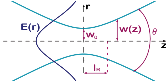
Figure II.2.: Schematic of a Gaussian beam with Rayleigh length l_R , waist w_0 and divergence angle \theta
