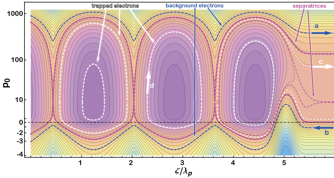
Figure III.3.: Phase space of a plasma wave in a co-moving frame with parameters as in fig. III.2 (top, a_0 = 3 ), but \beta_{p,ph} = 0.993 . The laser pulse sits at \chi/\lambda_p = 5
