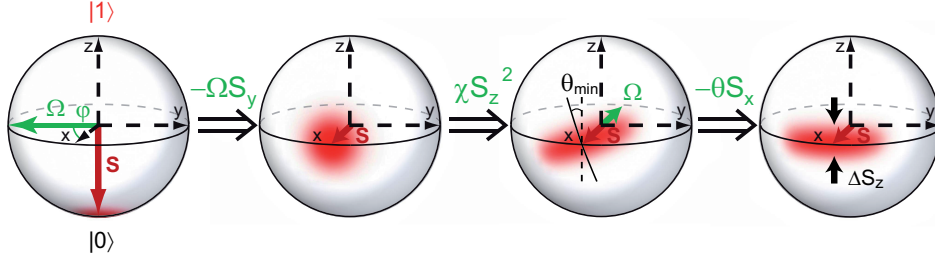
Figure 2.3: Squeezing sequence. Evolution of the BEC internal state on the Bloch sphere ( \delta = 0 for illustration). Starting with all atoms in |0\rangle , a \frac{\pi}{2} -pulse prepares a coherent spin state with mean spin \langle \mathbf{S} \rangle along x and isotropic quantum noise in the yz -plane (fuzzy red circle). Subsequent nonlinear evolution with \chi S_z^2 deforms the noise circle into an ellipse, creating a spin-squeezed state with reduced noise at an angle \theta_{\min} . To measure the spin quadrature S_\theta = (\cos \theta) S_z - (\sin \theta) S_y , a second pulse rotates the state around -x by a variable angle \theta , followed by detection of S_z .
