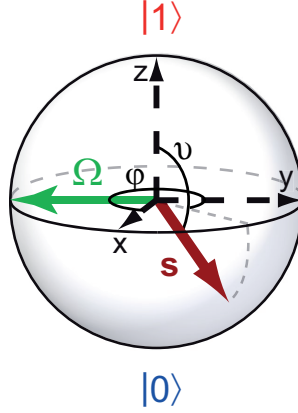
Figure 2.1: Bloch sphere. with an Bloch vector \mathbf{s} and a Rabi vector \Omega with \delta = 0 and \Omega_R = -i/2 . The angles \nu and \varphi characterizing the state are indicated.
