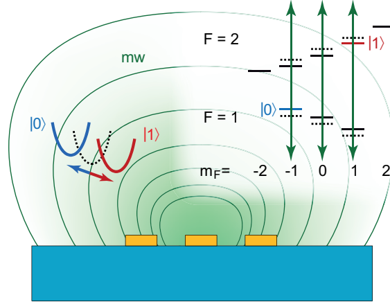
Figure 1.7: Schematic of the state-selective microwave potential.
