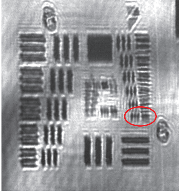
Figure 3.16: Imaging resolution , measured with an 1951 USAF optical calibration target. The group indicated by the red circle consists of three lines, each 2.2 \mu\text{m} wide and spaced by 2.2 \mu\text{m} ( 228 \text{ lp/mm} ) and can still be resolved by the objective. Reflections of the laser light used to image the target on the glass substrate result in double images (especially pronounced at the number 7 in the top right corner). The circular intensity modulation of the imaging light (centered around the lower right corner) is due to diffraction of the laser light on the aperture, since this image was taken before we introduced the lens L2 (see figure 3.15).
