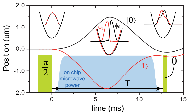
Figure 4.7: Experimental squeezing sequence. In between the pulses for internal-state manipulation (green), the state-dependent microwave potential is turned on (blue; pulse durations and microwave ramp times exaggerated for clarity). It dynamically splits and recombines the two BEC components, so that \chi > 0 during the time T . The simulated center-of-mass motion of the two states |0\rangle (black) and |1\rangle (red) is shown as a function of time. Insets: corresponding BEC mode functions \phi_0 and \phi_1 along the splitting direction in their respective potentials at the beginning, in the middle, and at the end of the sequence.
