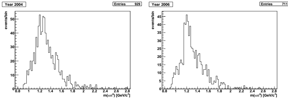
Figure A.1: \omega\pi^0 -mass (not acceptance corrected).
