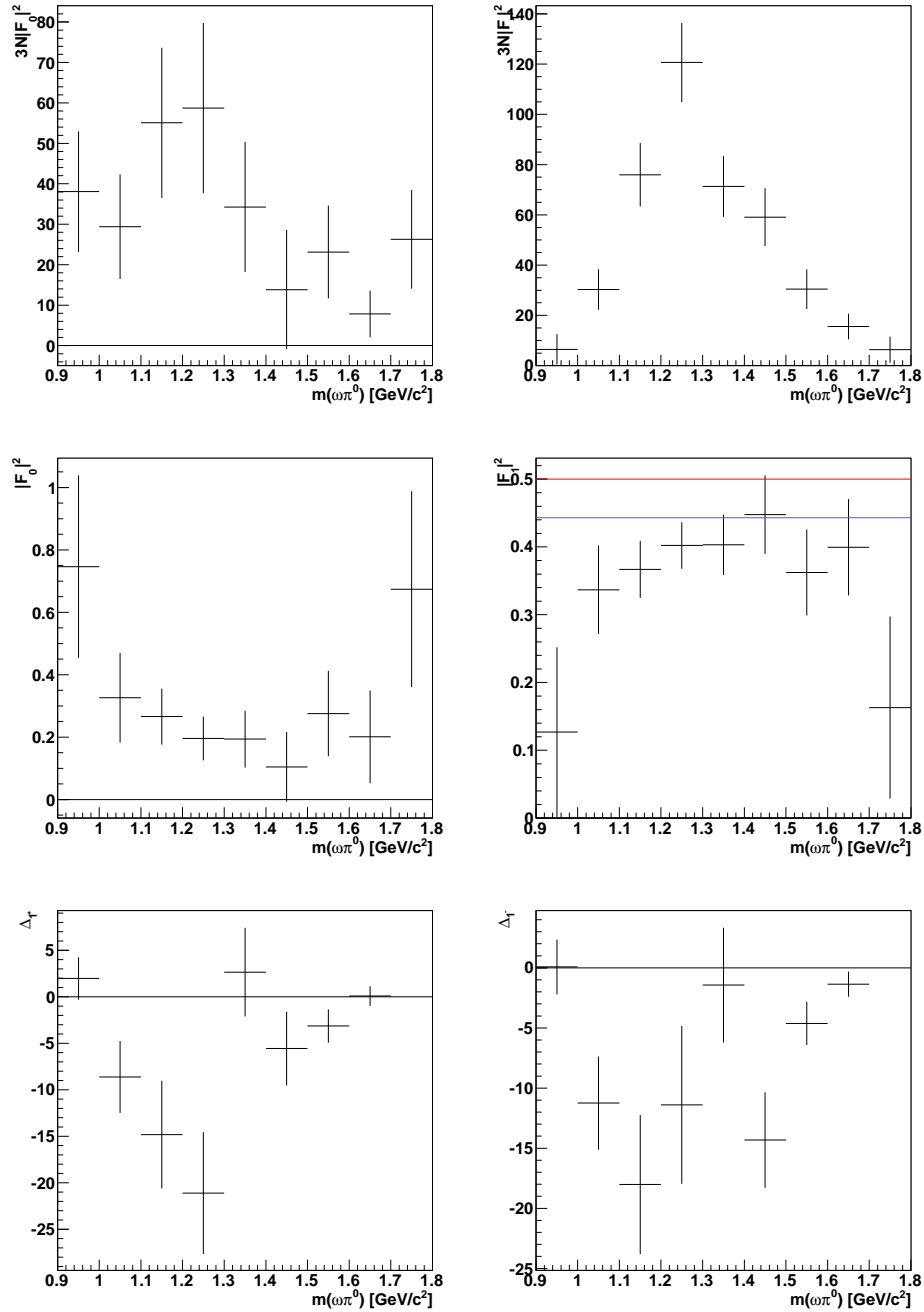
Figure 7.2: 3N|F_0|^2 , 3N|F_1|^2 , |F_0|^2 , |F_1|^2 , \Delta_{1+}(20) and \Delta_{1-}(20) for final sample with p_t^2 < 0.15 (\text{GeV}/c)^2 and \cos\theta < 0 . Corrected for acceptance. Red line: pure 1^- signal. Blue line: pure b_1(1235) .
